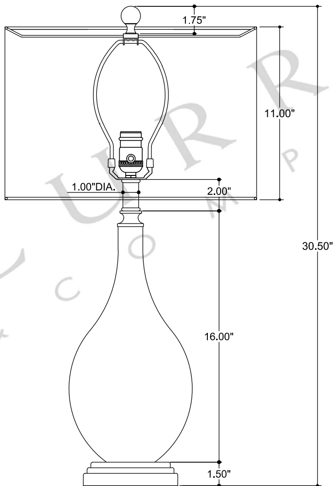
FRONT VIEW
